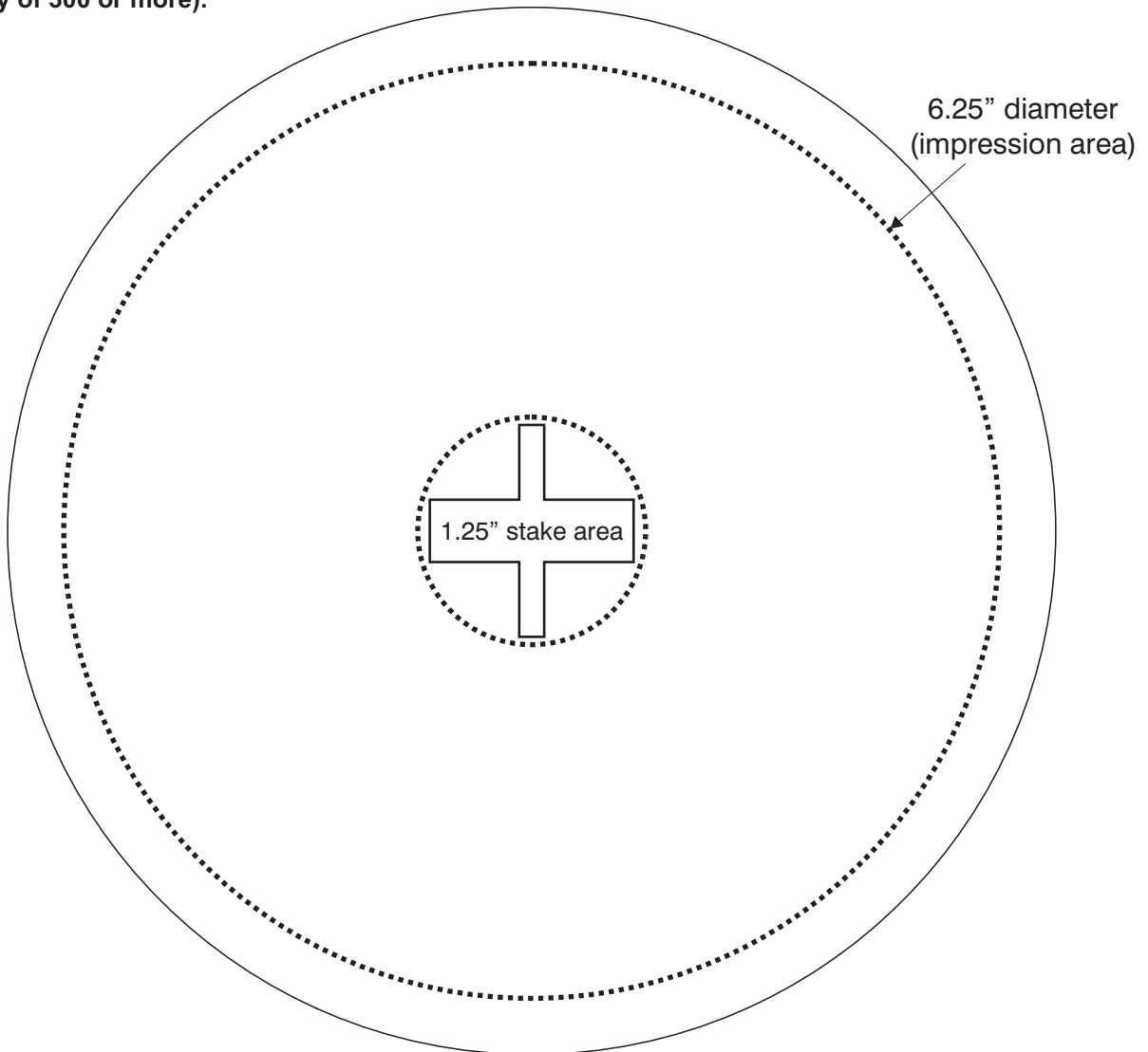
7" SOILMARKER TEMPLATE (REDUCED SIZE)
